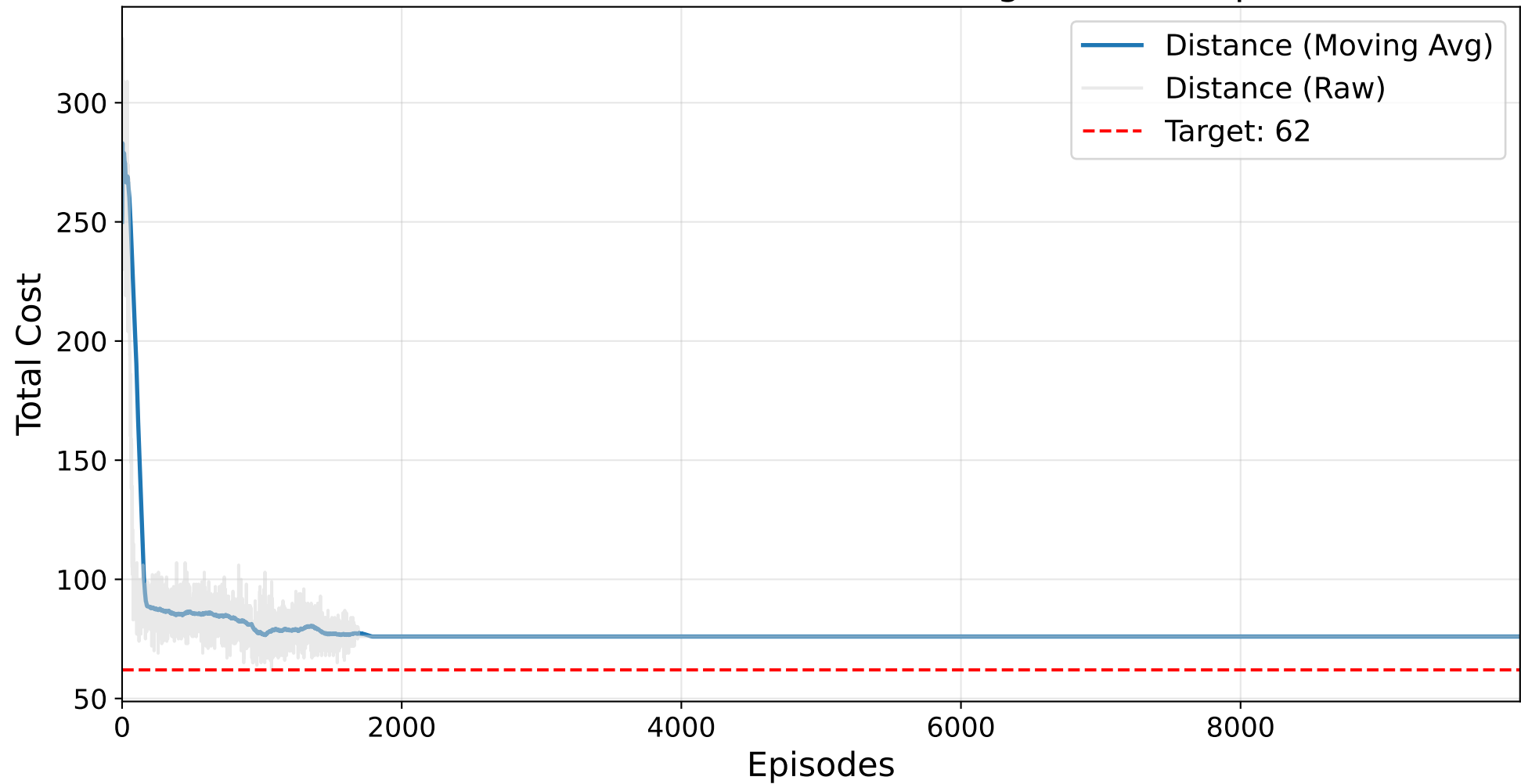
Final Masked AutoRL-SOP Training - ESC63.sop
